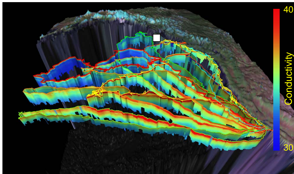
Figure 7. Conductivity profiles obtained from 7 northern elephant seal females as they migrated across the North Pacific from their rookery just north of Santa Cruz, CA.
