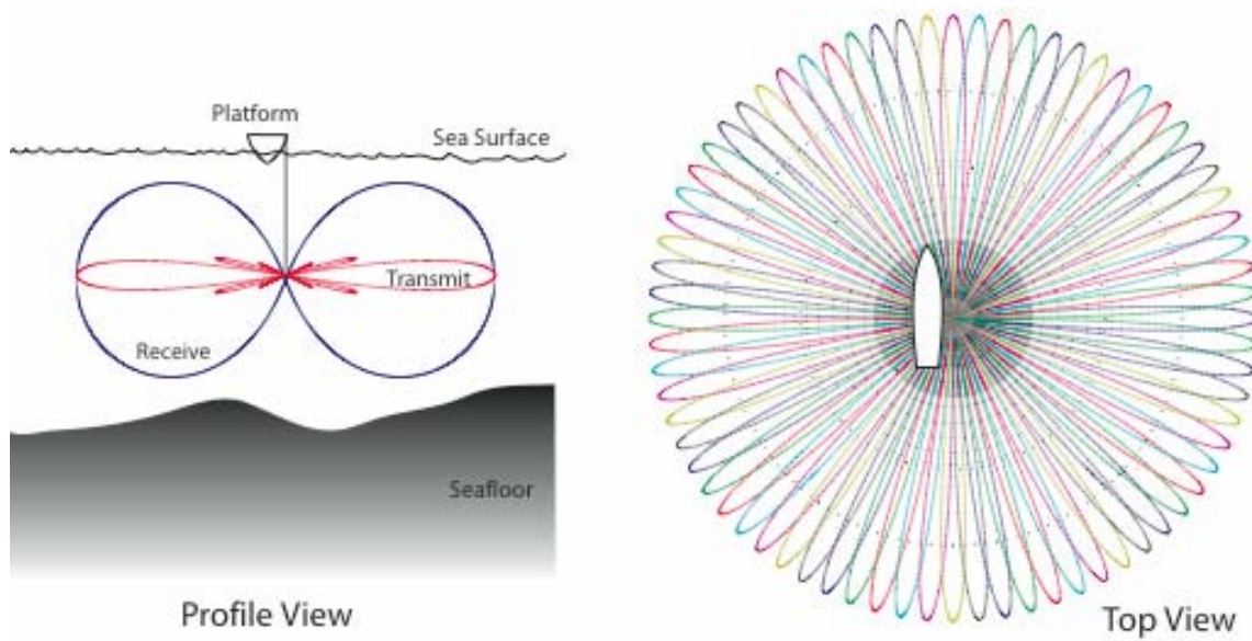
Figure 5: Deployment geometry and imaging volume of the mid-frequency circular array illustrating the receive and transmit beams patterns.
