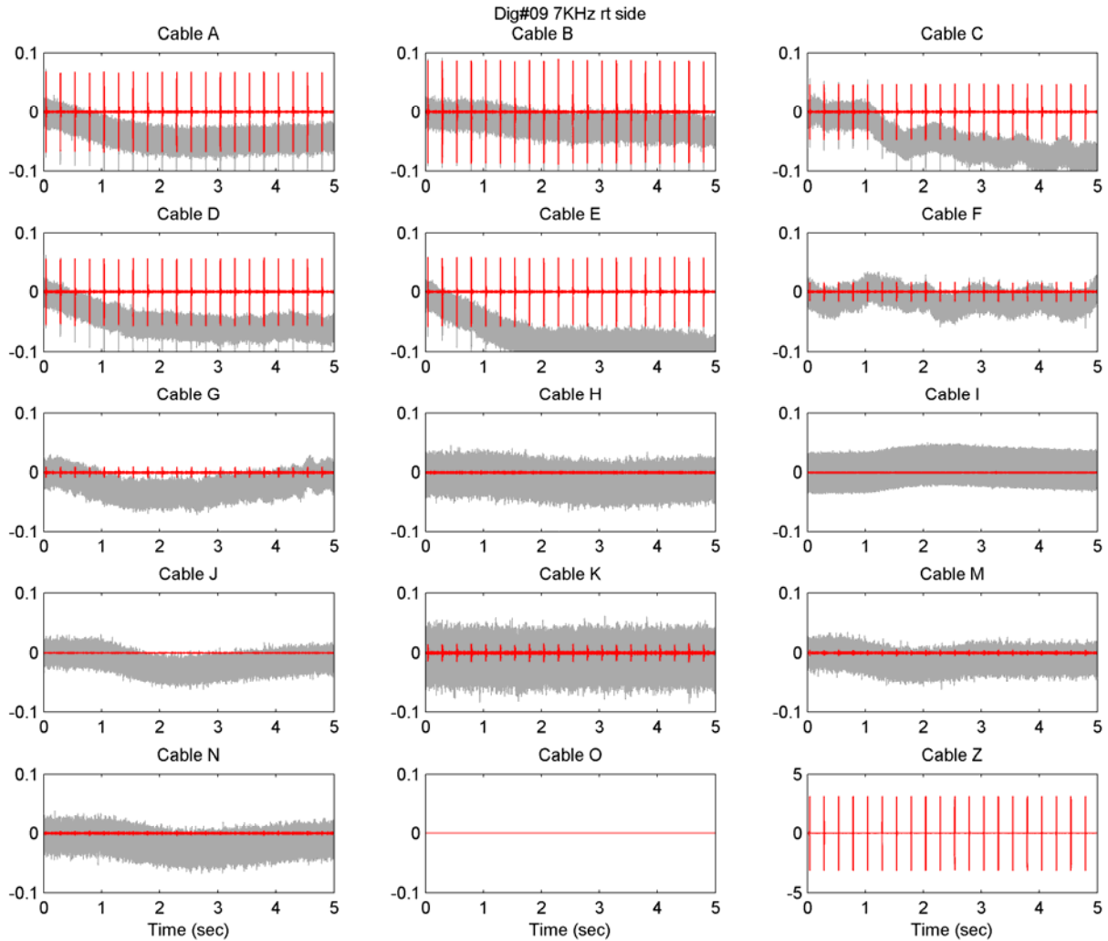
Fig. 3. Overview of acoustic data collected during the experiment with the common dolphin carcass at NSW Carderock Division on 4 February 2009 with the ITC-1032 spherical transducer on the right side of the carcass and transmit signal centered at 7 kHz. The total data collection time is 5 s; the pulse repetition frequency is 4 Hz. The total signal, including background noise, is shown in gray. The signal resulting from digital bandpass filtering with bandwidth equal to 10% of the center frequency is shown in red. Cables A, B, C, D, E, and G are connected to external sensors. Implanted sensors are connected to Cable F for the epaxial muscle near the dorsal fin, Cable H for the left lung, Cable I for the external right lung, Cable J in the rectal abdomen, Cable K for the melon, Cable M for the left lung, Cable N for the right lung, and Cable O along the right ear. Credit: Y.-T. Lin, M. Hastings, K. Rye, K. Foote.
