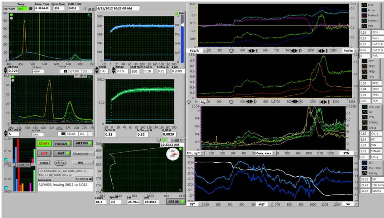
Fig. 8. A transect map (transect of interest highlighted in yellow) and a screenshot of the ALFA operational software taken during a cruise in the Gulf of Mexico with the ALFA instrument, May-June 2012. Right panels display spatial distributions of Chl a (green), CDOM (dark-blue, upper panel), Fv/Fm 405 nm excitation (magenta), Fv/Fm 514 nm excitation (teal), PBP pigments (yellow-orange), temperature (blue), and salinity (white).
