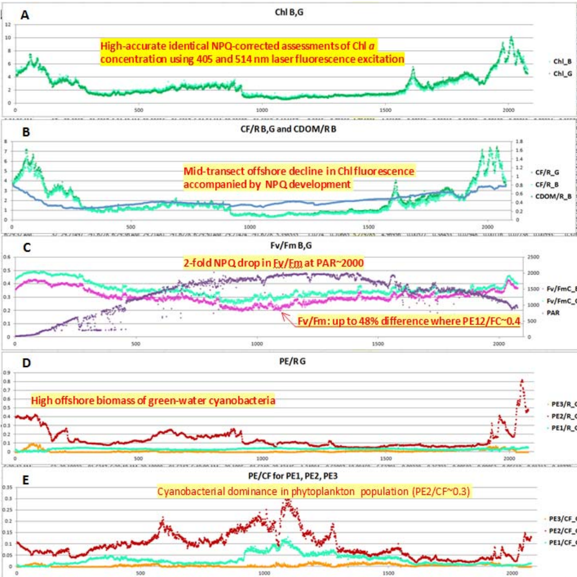
Fig. 6. Spatial distributions of the key fluorescence characteristics measured underway in the flow-through mode by the ALFA-X-405/514 instrument. The transect track is highlighted with yellow color in the map displayed in Fig. 5. The updated ALF analytical algorithms were refined and optimized to provide accurate assessments of chlorophyll (Chl) concentration (A), CDOM (B), variable fluorescence (phytoplankton physiological characteristic, C), and basic structural characterization of phytoplankton community structure (D, E).
