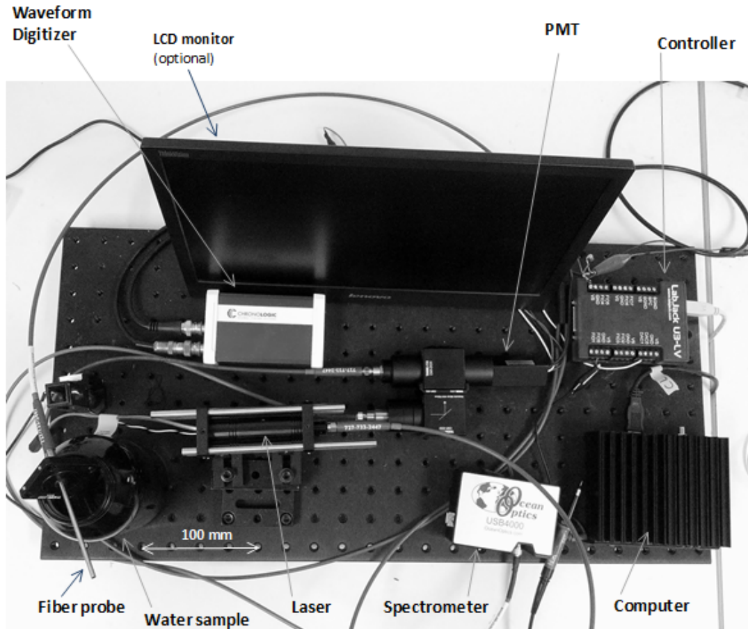
Fig. 10. Breadboard tests of the ALF-In Situ (ALFIS) instrument prototype designed by the LDEO ALF team in June-July 2012 (provisional patent application # 2413.141PRV of July 30, 2012). The use of the new 514 nm laser, fiber-probe and dichroic beamsplitter were critical design solutions for the ALFIS prototype development. The Wet Labs and LDEO ALF project teams are currently building on this basis an operational ALFIS instrument to conduct its field tests in Spring 2013.
