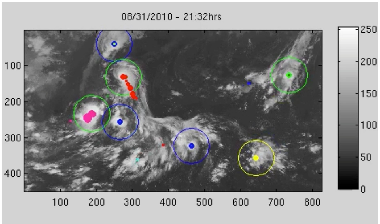
Snapshot of the automatic tracking system with several identified storms being tracked in the western North Pacific basin for the date and time indicated on the top of the image. The brightness temperature is given in an 8-bit digitized format (0--255). The latitude, vertical axis, and longitude, horizontal axis, are given in image pixels.
