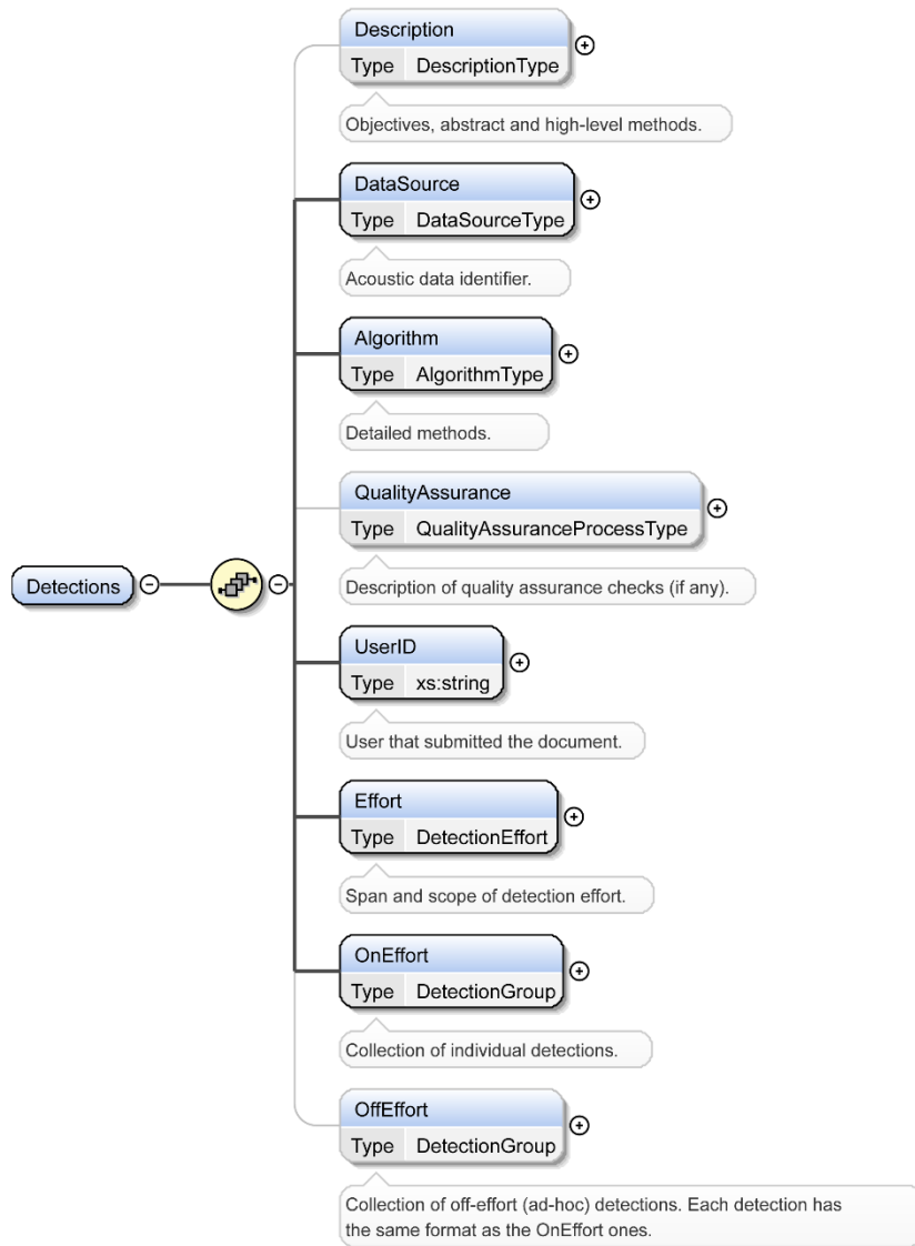
Figure 2 – Top level view of the schema for a detections document.
