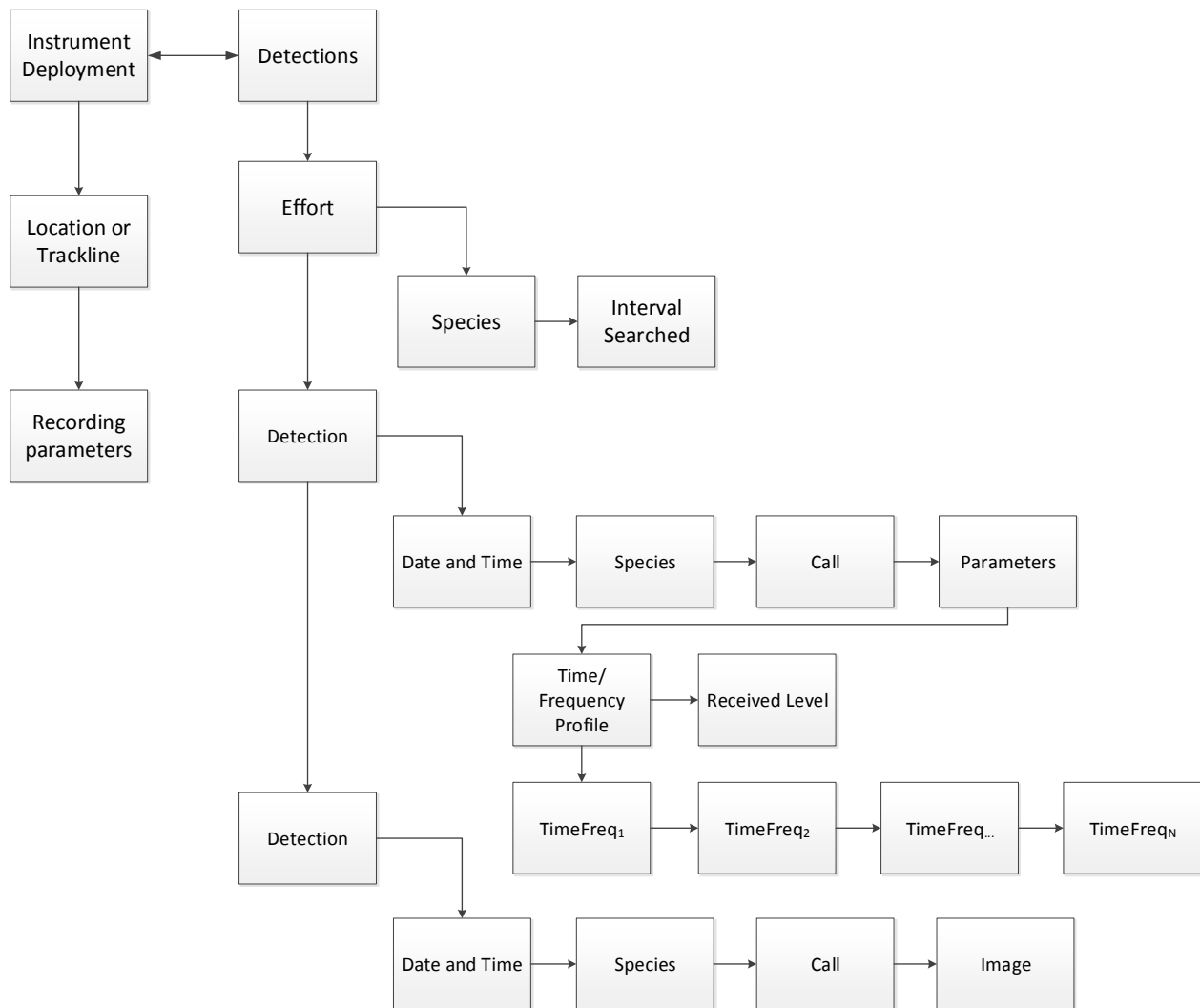
Figure 1 - A network data model provides linkages between different types of data
