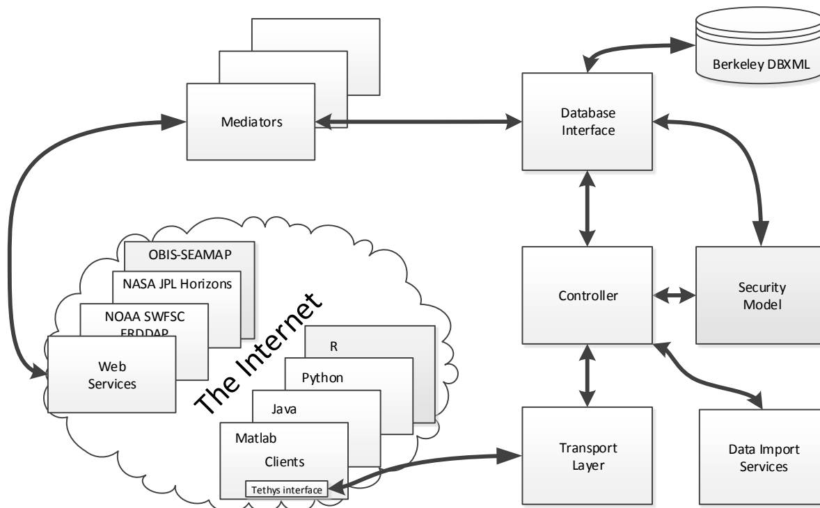
Figure 4 – Tethys reference implementation architecture
