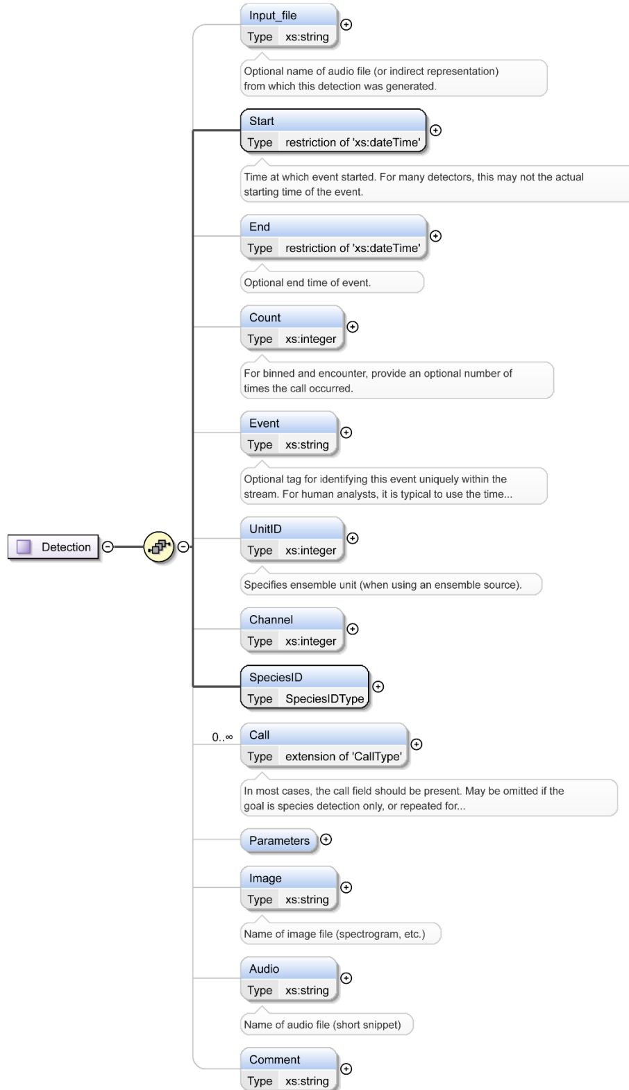
Figure 3 – Schema for individual detections.
