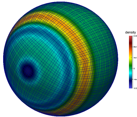
Figure 3: Simulation on the GPU: Acoustic wave propagating on the sphere at the speed of sound is simulated using the GPU on a cubed sphere grid. The result after 5 hours is shown.
