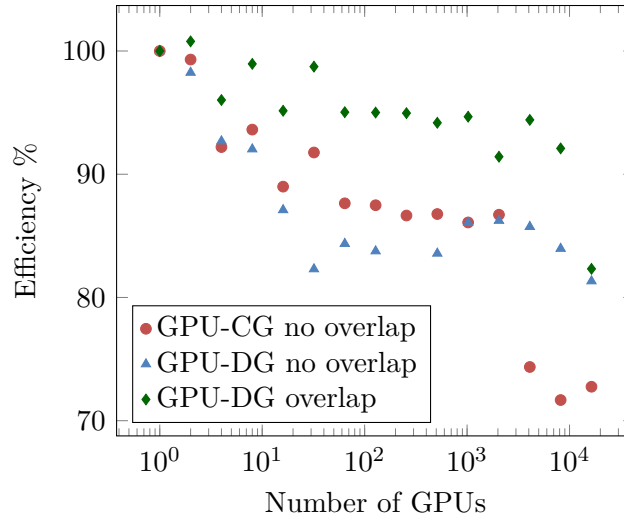
Figure 2: Scalability test of Multi-GPU implementation of NUMA: Weak Scalability of NUMA (running explicit time-steps) for up to 16384 GPUs on the Titan supercomputer is shown. Each node of Titan contains a Tesla K20 GPU. The test is conducted using the unified implementation of CG and DG with and without the overlapping of communication with computation. DG benefits from overlapping of communication with computation as the figure clearly shows; overlapping helps by hiding latency of communication between the CPU and GPU.
